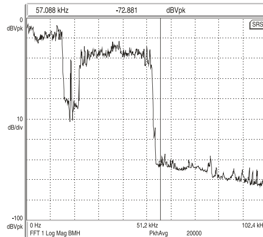
Figure 5-1: Typical 5750 HD baseband spectrum with heavy processing, 0-100 kHz.
